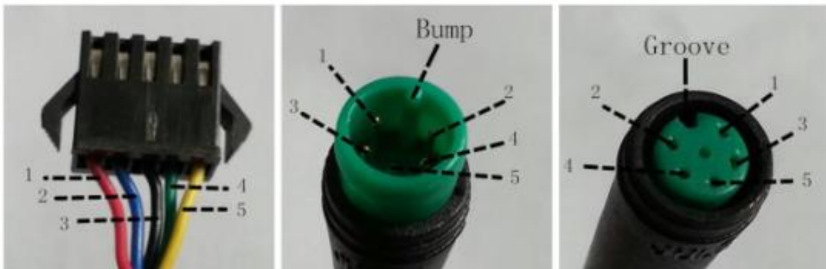
Display-side Connector
